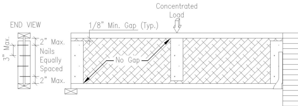
FIGURE 2—WEB STIFFENERS
